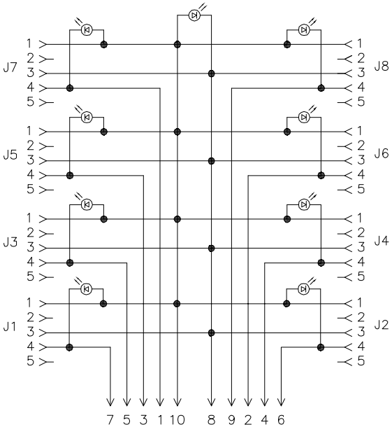
WIRING DIAGRAM
